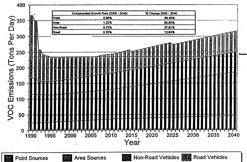
Figure 1: Portland-Vancouver Ozone Precursors Human caused emissions: 1990-2040
