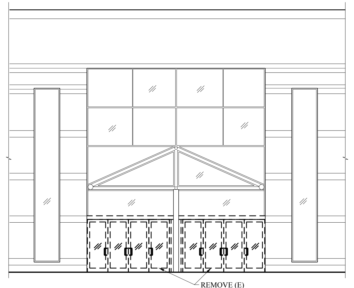
AWNING ENTRY DEMO ELEVATION
