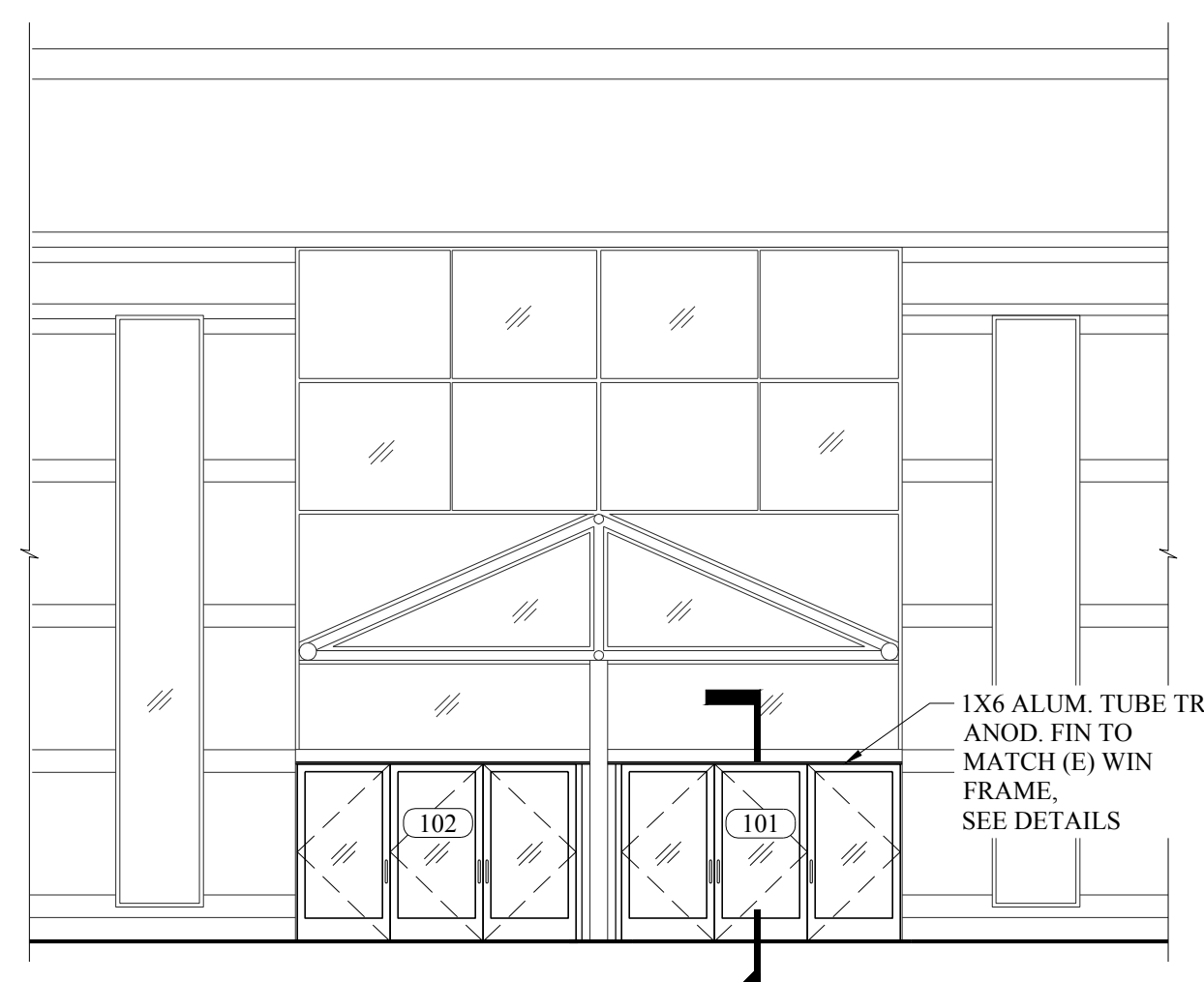
AWNING ENTRY PROPOSED ELEVATION
