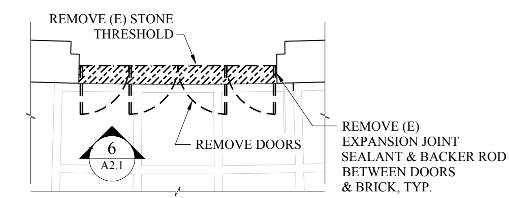
MID-ENTRY DEMO PLAN
