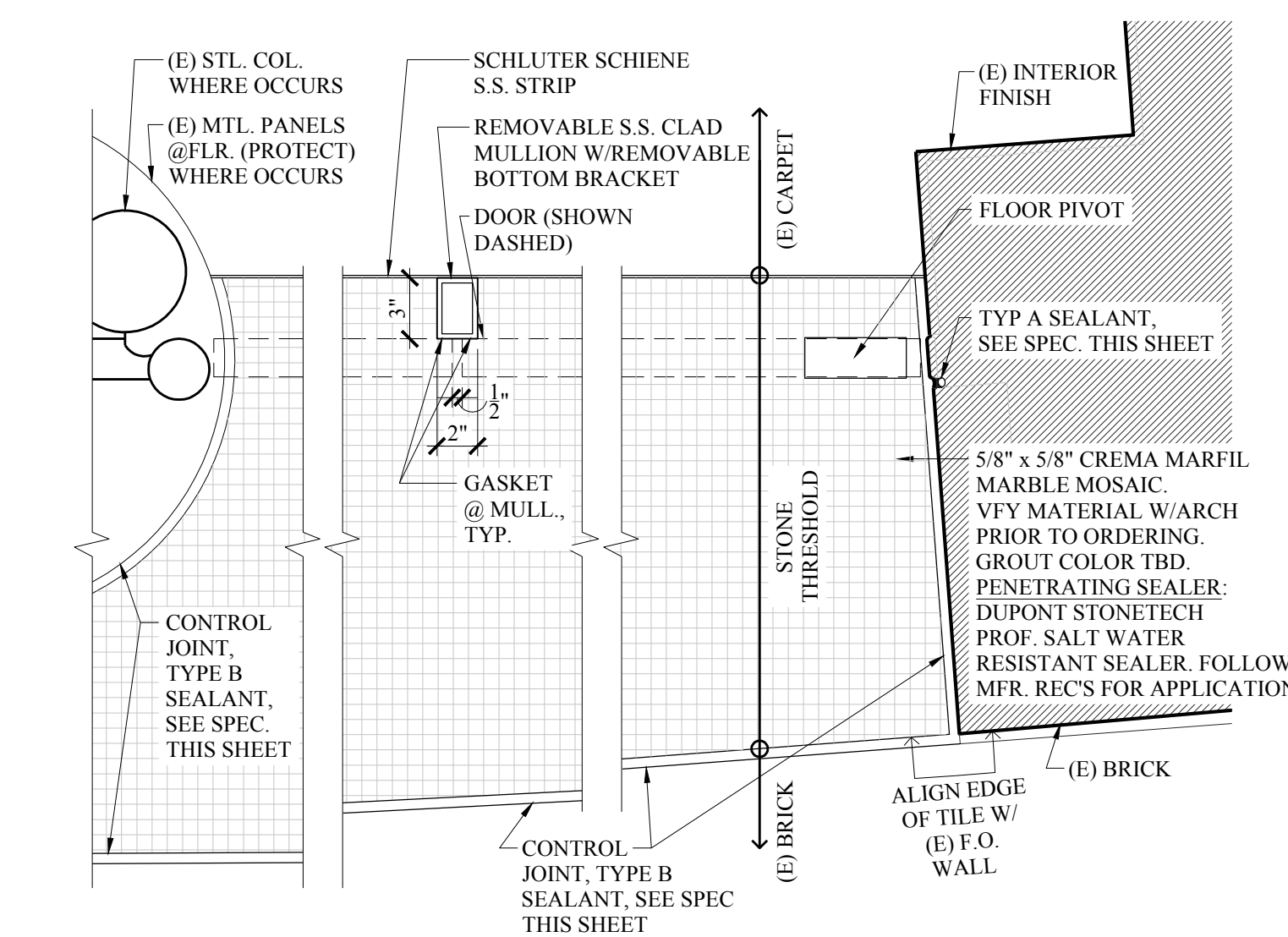
THRESHOLD PLAN DETAIL
