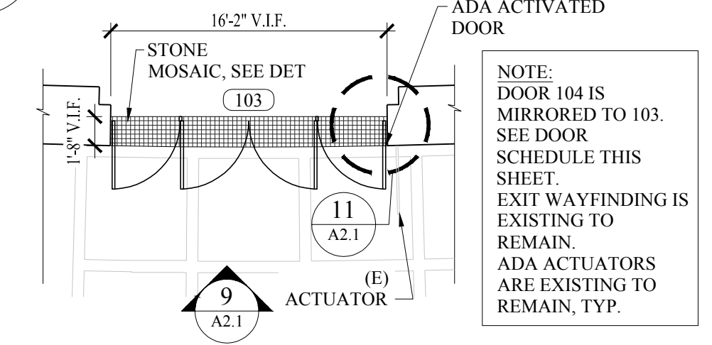
MID-ENTRY PROPOSED PLAN
