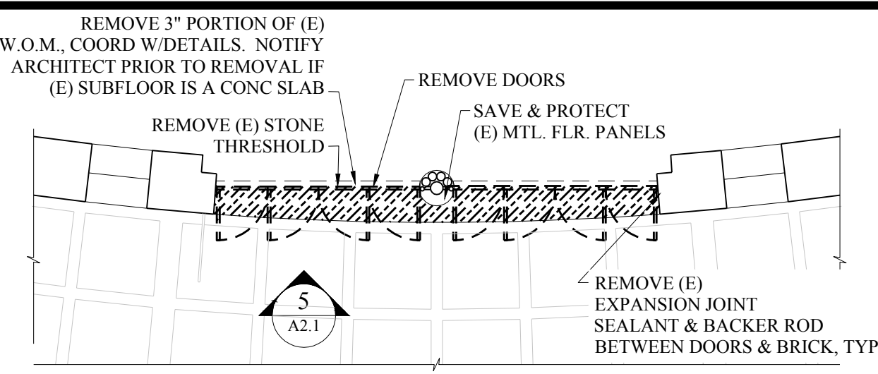
AWNING ENTRY DEMO PLAN
