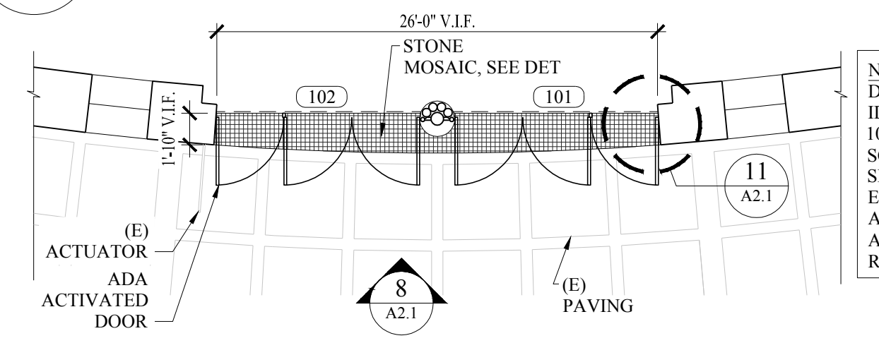
AWNING ENTRY PROPOSED PLAN
