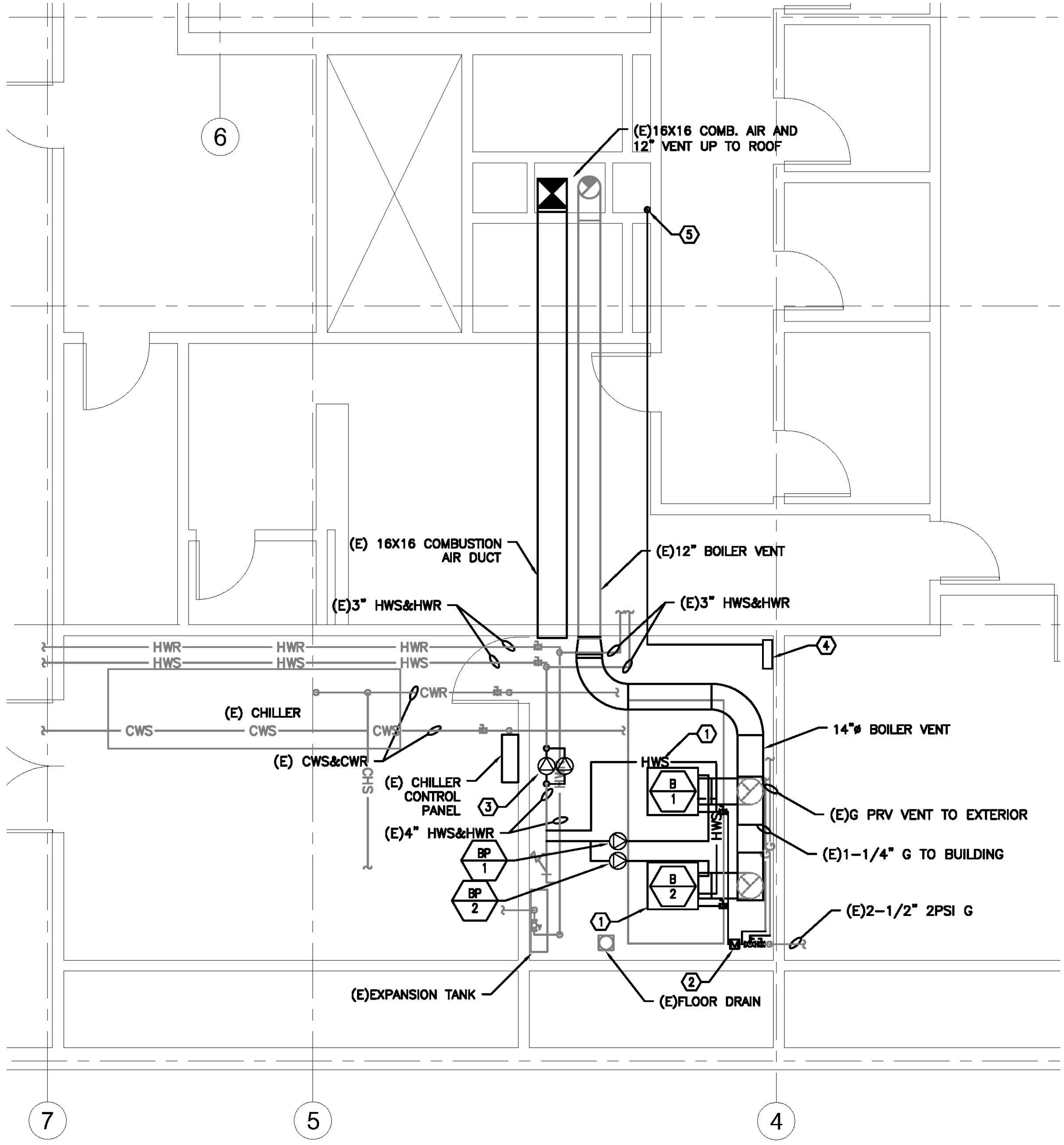
2 BOILER ROOM PLAN M2.1 SCALE: 1/4" = 1'-0"
