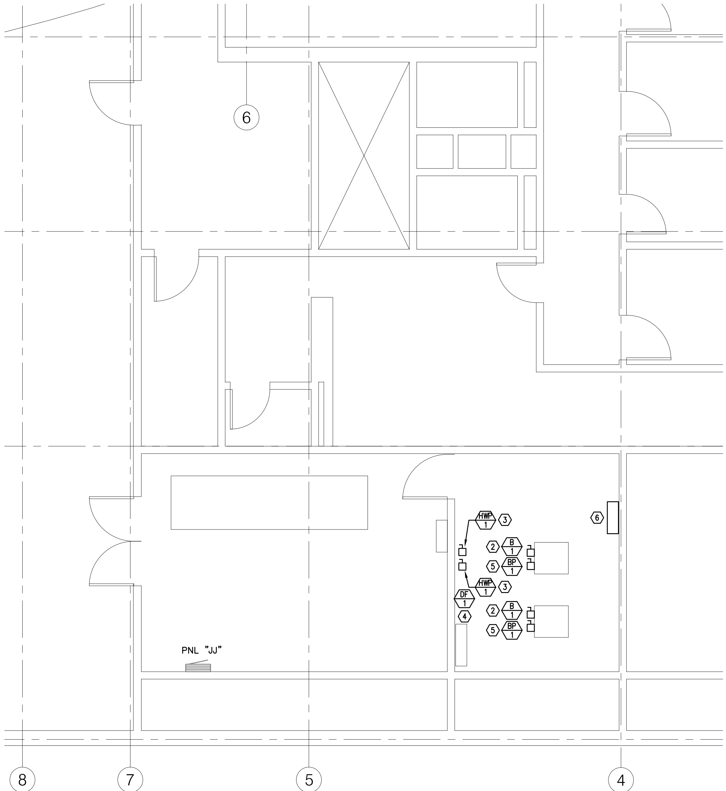
2 BOILER ROOM PLAN E2.1 SCALE: 1/4" = 1'-0"
