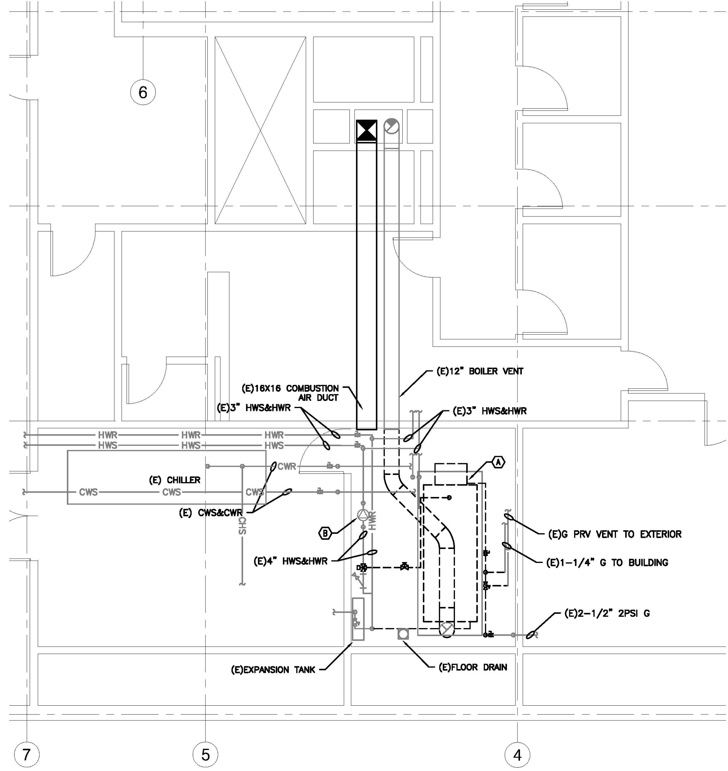
1 BOILER ROOM DEMO PLAN M2.1 SCALE: 1/4" = 1'-0"
