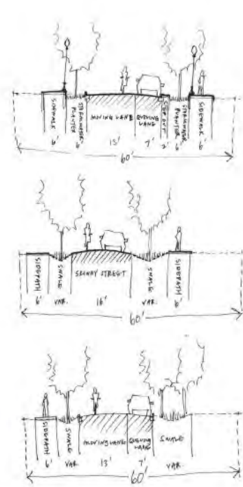
Conceptual cross-sections of SW 53 rd Ave
