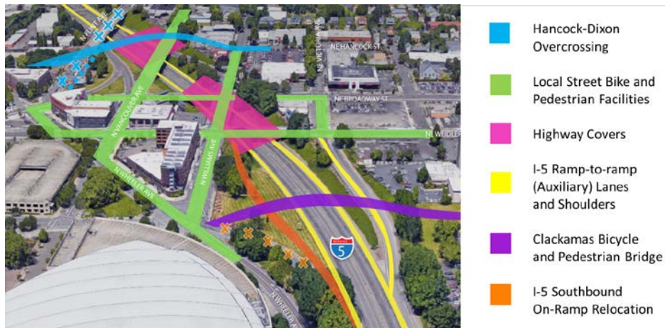
Figure 8.4: I-5/Rose Quarter Project Features
