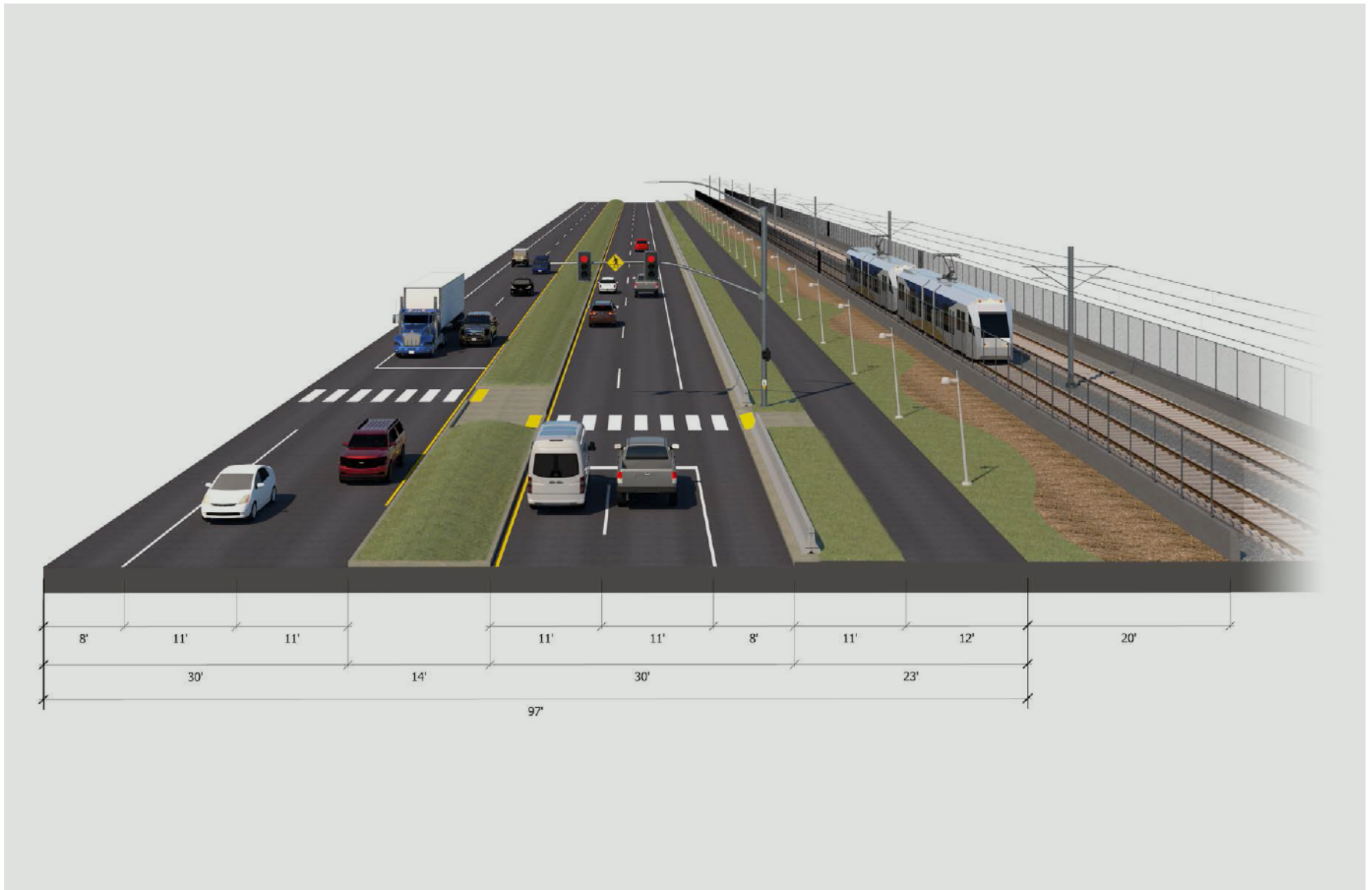
Highway cross-section
