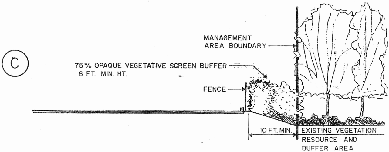
VEGETATIVE SCREENING FIGURE 6
