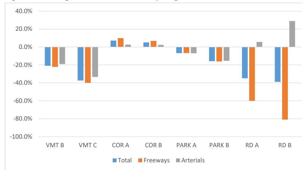
Figure 1.4-6 Change in Vehicle Hours of Delay - Region
