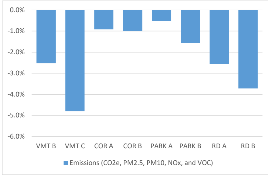
Figure 1.4-11. Change in Emissions - Region
