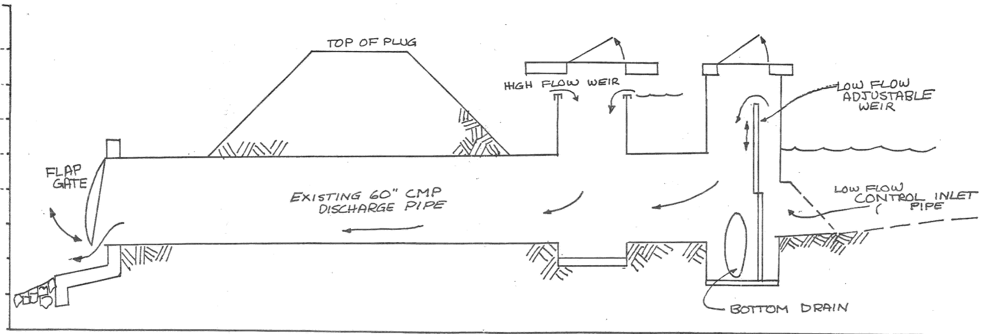
SMITH & BYBEE LAKES OUTFALL CONTROL STRUCTURE
