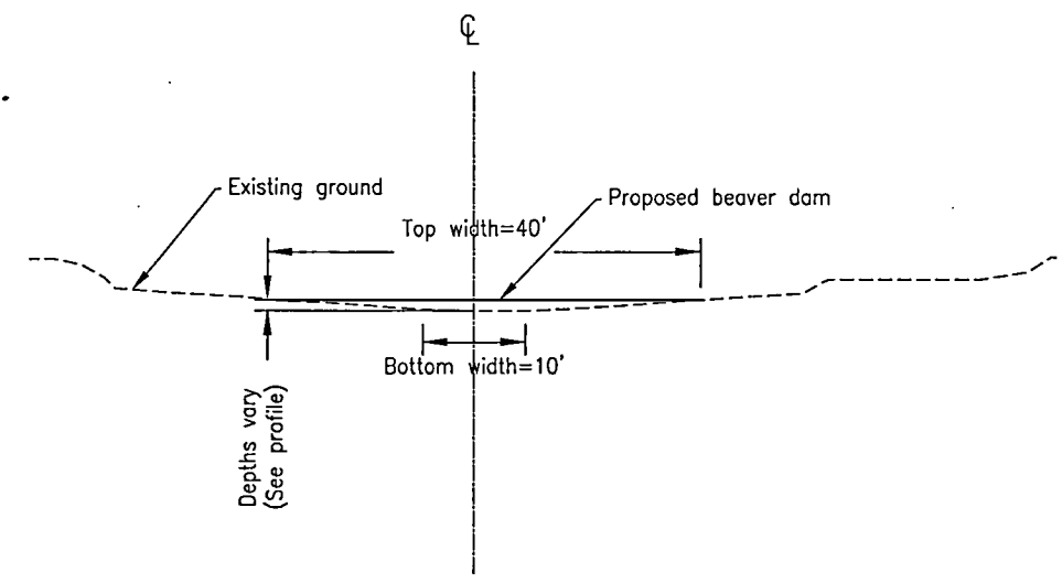
Section B (NTS) Sta. 24+94 to 25+08
