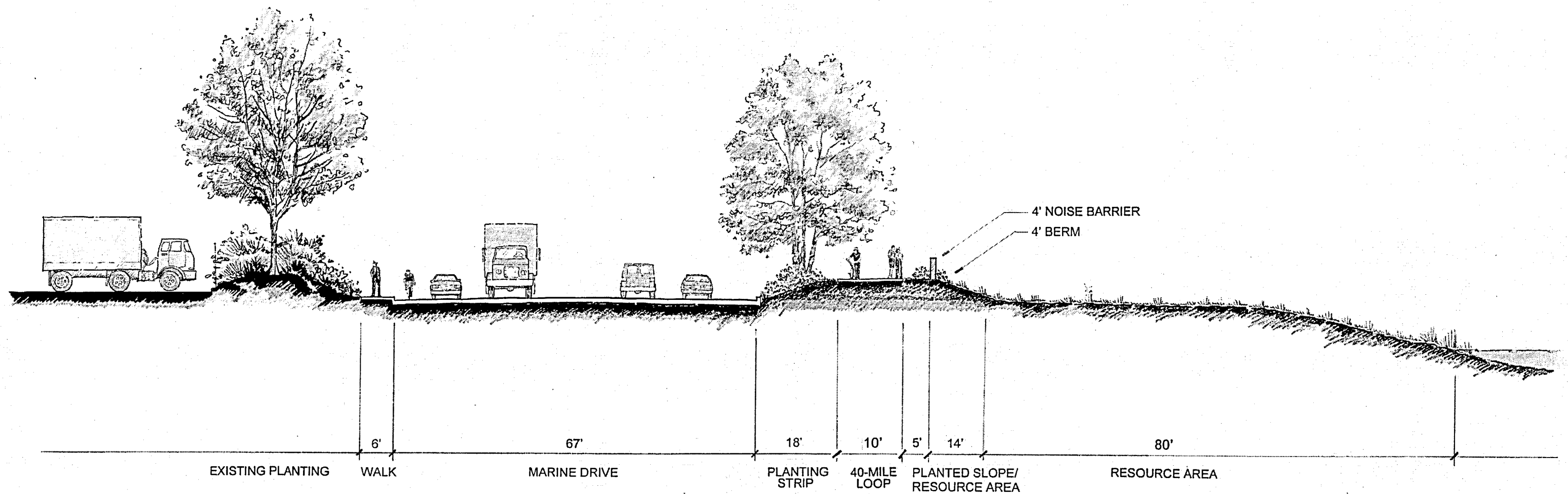
Earthen Berm with Noise Barrier
